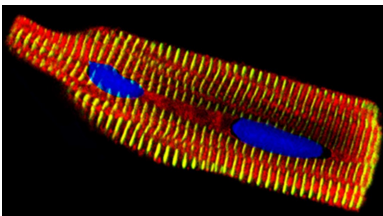
Cardiomyocyte showing positions of nuclei (blue) and two sarcomeric proteins (red and yellow).
