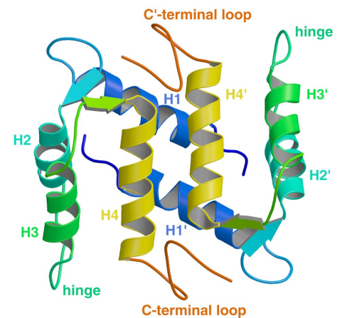
3D structure of Metastasis Protein 1 (mts1) determined by NMR
